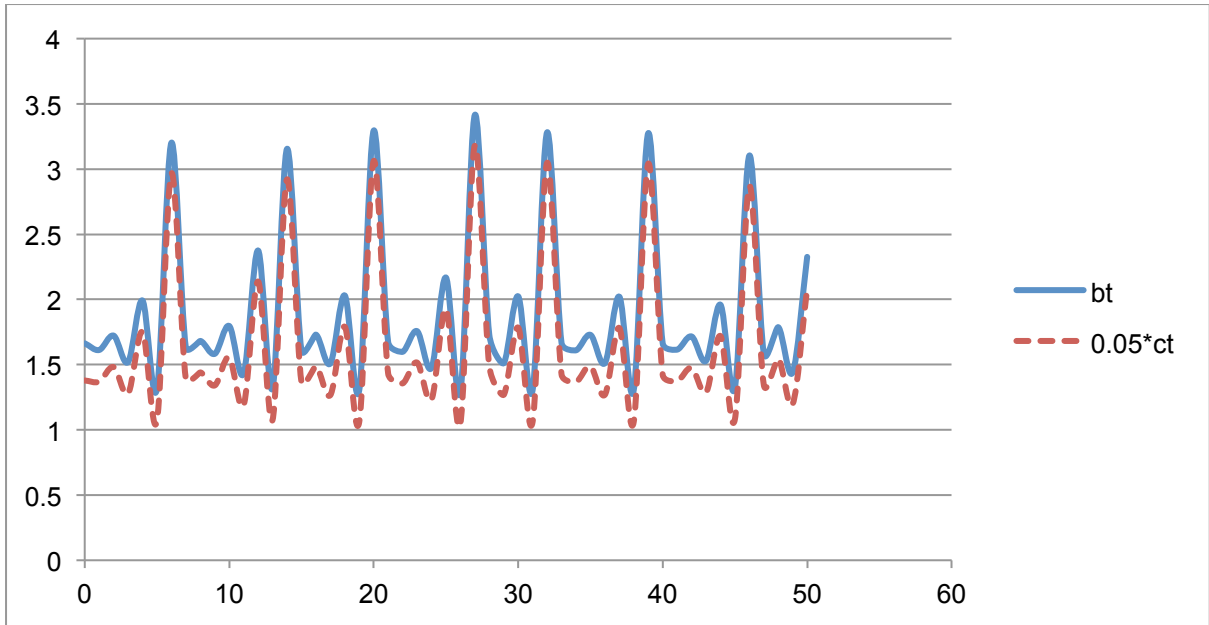
Slight change in initial condition
