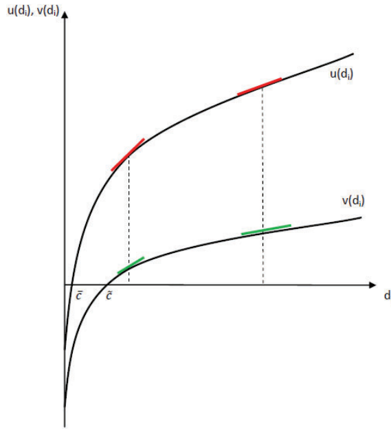
Figure 1: State-dependent utility functions u(\cdot) and v(\cdot) .
